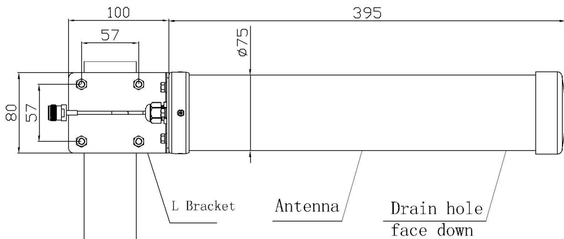
Installation sketch
